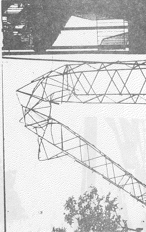
Photo 6 - Several lattice towers of this type collapsed in David, Gilbert and Hugo (David)
