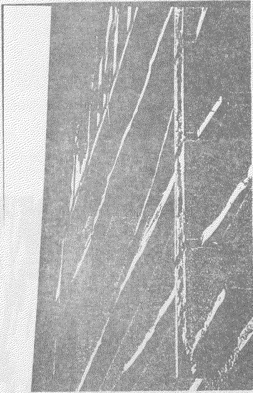
Photo 9 - Longitudinal splitting of timber rafters (Hugo)
